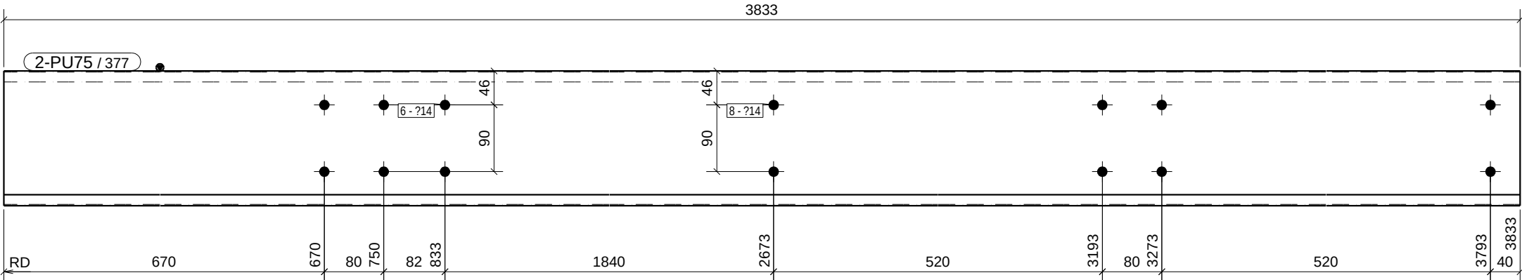
FRONT VIEW
